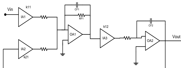
Fig. 1. Implementation of a biquadratic section in the device ispPAC10.
